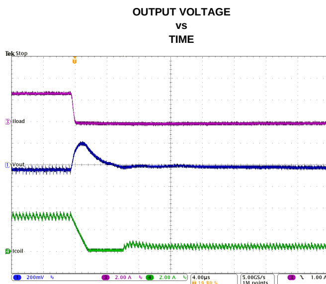
Figure 32. Load Transient Response of Figure 30, falling edge
